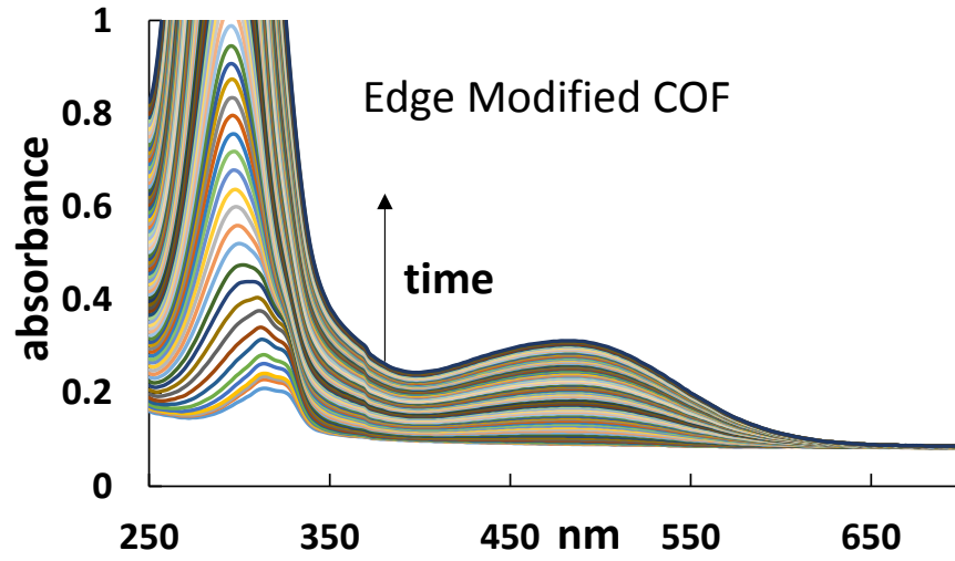
Figure E.3 UV Vis Spectra of Edge Modified COF.
