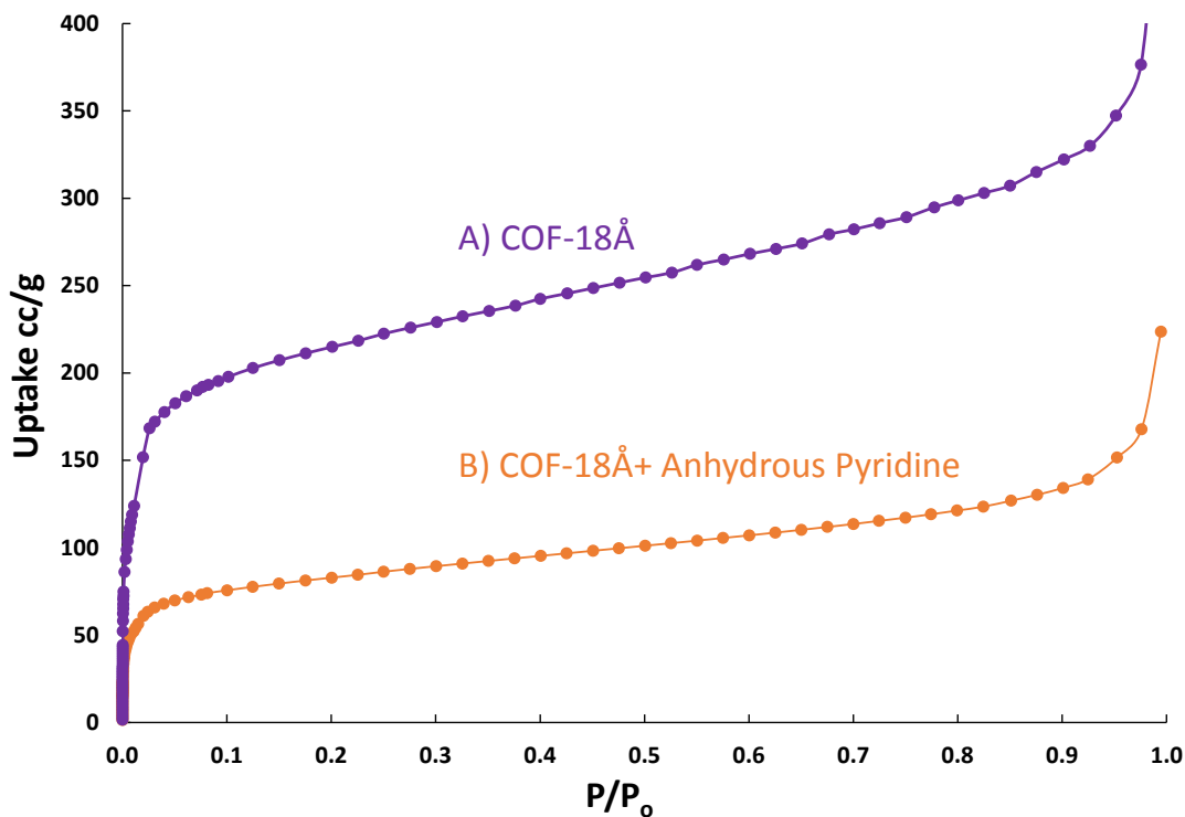
Figure 3.10 Nitrogen Adsorption of pristine A)COF-18Å and B) COF-18Å + Anhydrous Pyridine.
