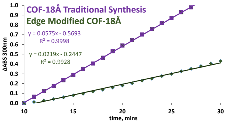
Figure 4.10 Relative stability of COF-18 Å vs edge modified material.
