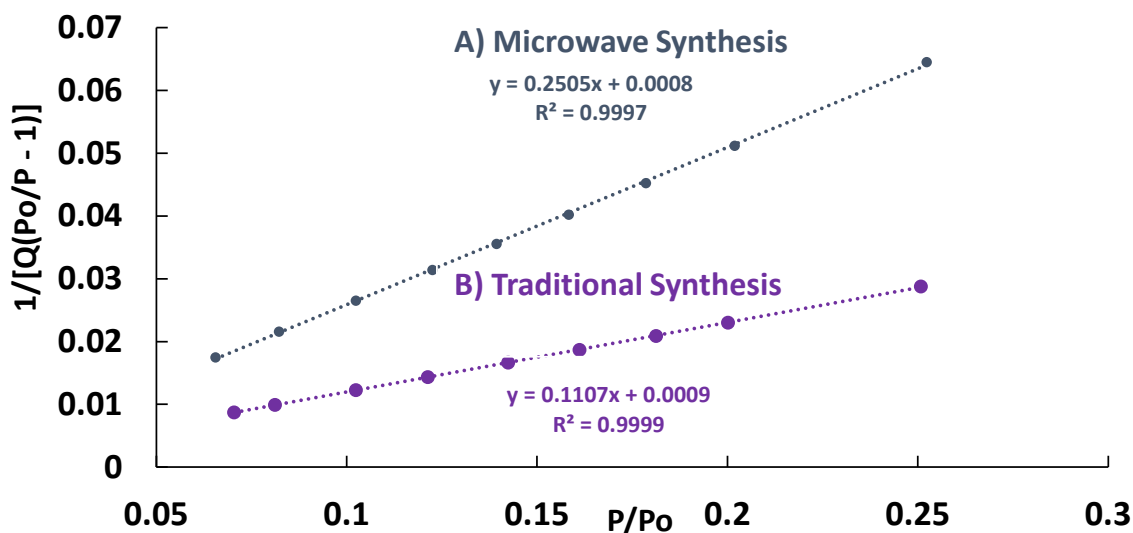
Figure 2.6 BET treatment from the Nitrogen isotherms of A) microwave synthesized COF-18Å, and B) traditionally synthesized COF-18Å.
