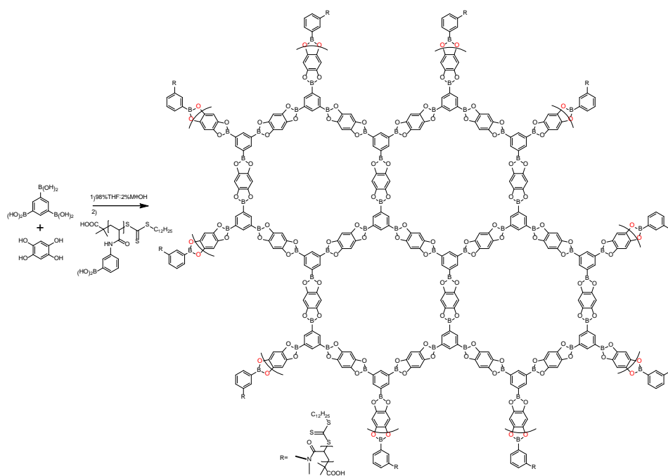
Figure 4.7 Edge Modified COF-18Å Synthetic Scheme.
